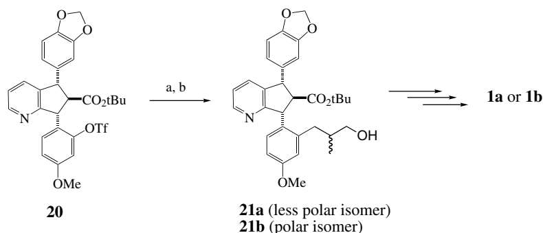
Scheme 2. Introduction of 3-hydroxy-2-methylpropyl group. Reagents and conditions: (a) methallyl alcohol (10 equiv), \text{PdCl}_2(\text{PPh}_3)_2 (10 mol%), \text{NaHCO}_3 (2 equiv), DMF, 130^{\circ}\text{C} , 12 h; (b) \text{NaBH}_4 , MeOH, rt.
