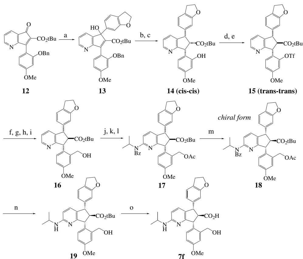
Scheme 1. The representative synthetic route: synthesis of 7f . Reagents and conditions: (a) 5-bromo-2,3-dihydrobenzo[ b ]furan, Mg, THF, -78^{\circ}\text{C} , 89%; (b) \text{Ac}_2\text{O} , DMAP, \text{CHCl}_3 ; (c) \text{H}_2 , \text{Pd}(\text{OH})_2 , \text{NaHCO}_3 , THF–EtOH, rt, 82% in two steps; (d) t\text{-BuOK} , t\text{-BuOH} –THF, 0^{\circ}\text{C} ; (e) \text{Tf}_2\text{O} , DMAP, \text{CHCl}_3 , 0^{\circ}\text{C} , 72% in two steps; (f) vinyl(tributyl)tin, \text{PdCl}_2(\text{PPh}_3)_2 , DMF, 125^{\circ}\text{C} , quant.; (g) \text{OsO}_4 , NMO, THF– \text{H}_2\text{O} , rt; (h) \text{NaIO}_4 , THF– \text{H}_2\text{O} , rt; (i) \text{NaBH}_4 , THF– \text{H}_2\text{O} , 75% in three steps; (j) \text{Ac}_2\text{O} , DMAP, THF, rt; (k) m -CPBA, \text{CHCl}_3 , 0^{\circ}\text{C} ; (l) i\text{PrN}=\text{C}(\text{Cl})\text{Ph} , \text{Et}_3\text{N} , \text{CHCl}_3 , 70^{\circ}\text{C} ; (m) optical resolution using Chiralpak AD, hexane-2-propanol, 33% from 16 ; (n) DIBAL, THF, -78^{\circ}\text{C} , 91%; (o) TFA, rt, 92%.
